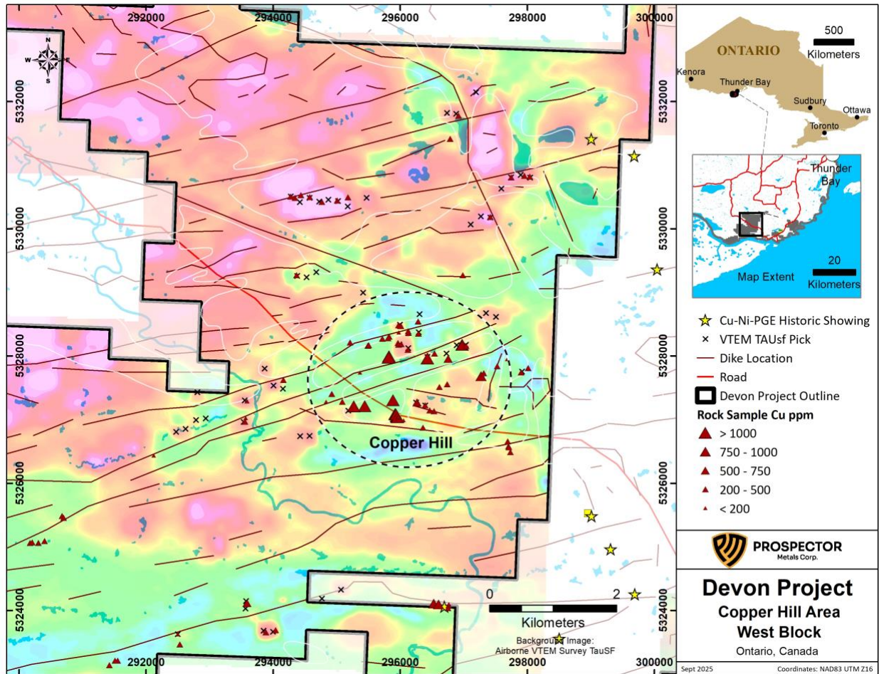
Figure 1: Surface grab samples overlaying the VTEM
